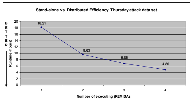
Figure 14. Data decomposition-based distributed execution: efficiency vs. number of executing jREMISAs.
