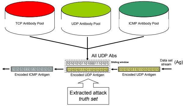
Figure 4. Transient (data set) Ags evaluated against its IP protocol-matching Ab.
