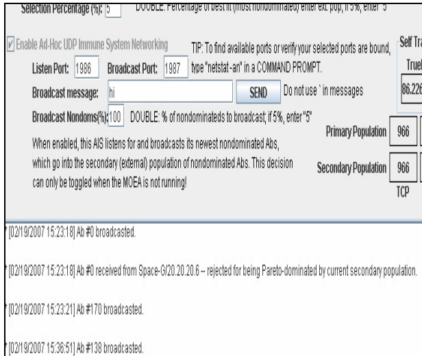
Figure 11. Snapshot of jREMISA distributed communication.
