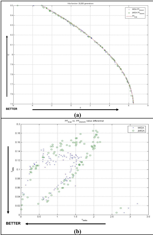
Figure 7. (a) MISA and jMISA PF vs. MISA's true PF^* ; (b) Euclidian distance measure of MISA and jMISA points from MISA's true PF^* .
