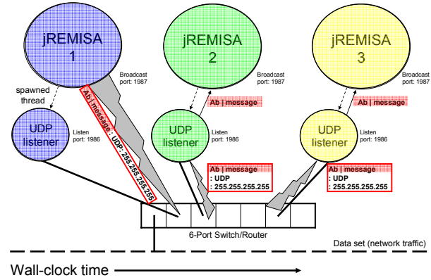
Figure 5. jREMISA distributed communication architecture.
