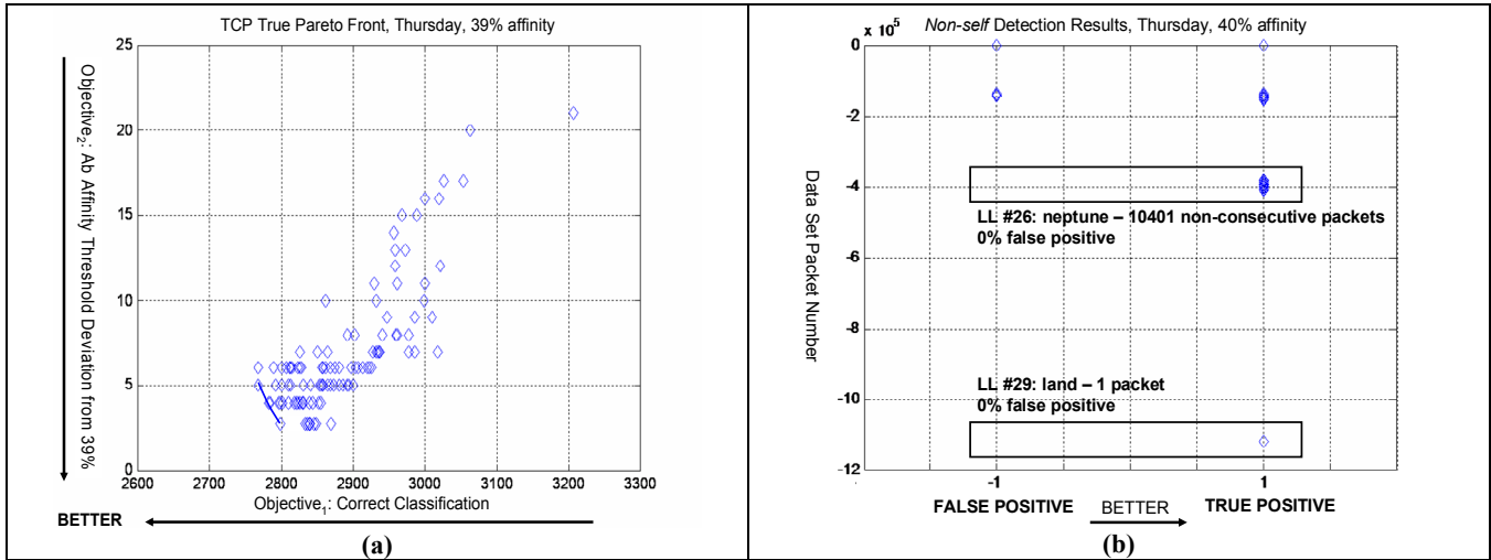
Figure 10. MOEA post-execution: (a) TCP pop, PF^* ; (b) attack graph: two attacks found with 0% false positive rate.
