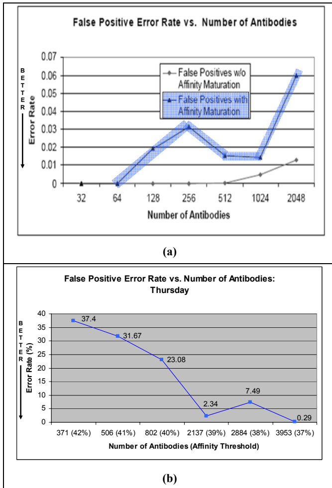
Figure 15. false positive error rate trend: (a) Warthog [15] vs. (b) jREMISA.
