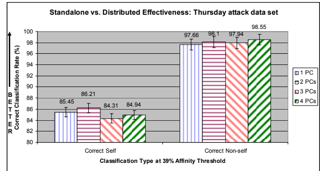
Figure 13. Standalone vs. distributed effectiveness against the week-two Thursday insider attack data set.
