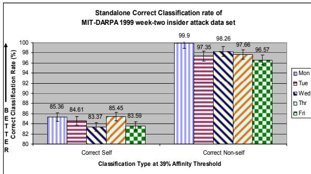
Figure 12. jREMISA standalone effectiveness against each day of the week-two insider attack data set.
